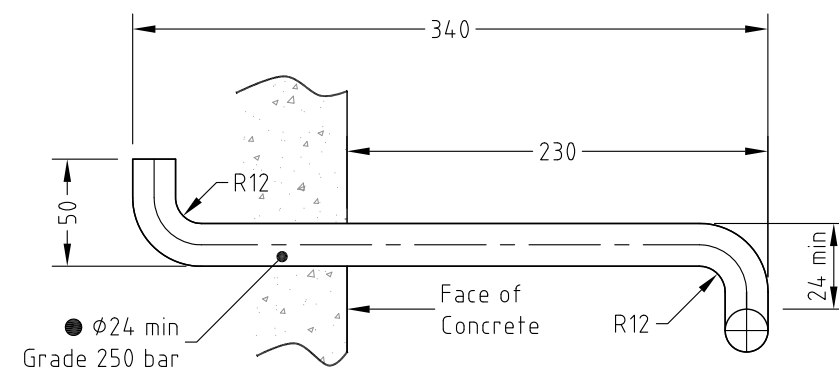
SECTION B SCALE NTS
